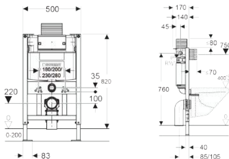
Alpha12 Concealed Cistern with Duofix 224.049.00.1
