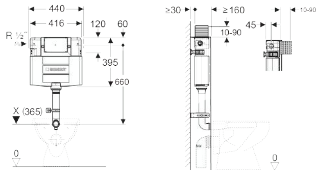
Alpha12 Concealed Cistern Mid Level 224.039.00.1
