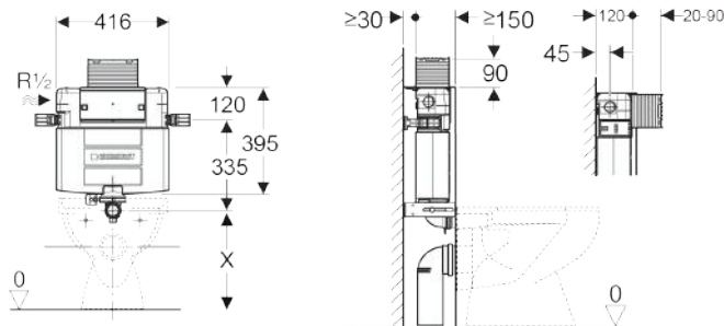
Alpha12 Concealed Cistern Low Level 224.038.00.1
