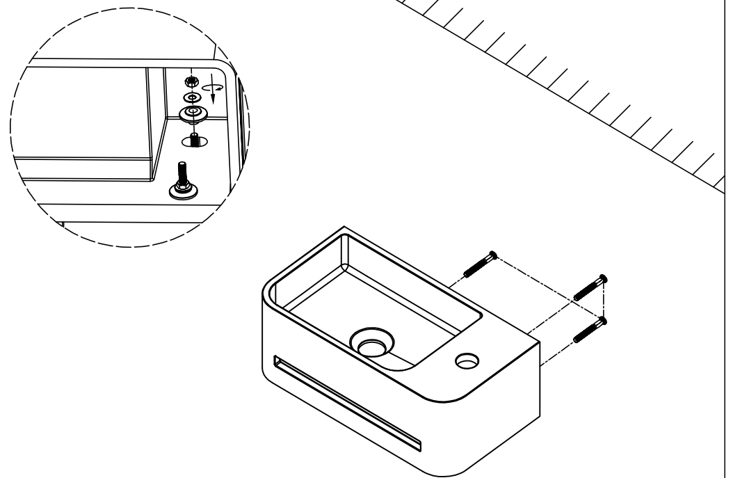
Expansion screws x 3
