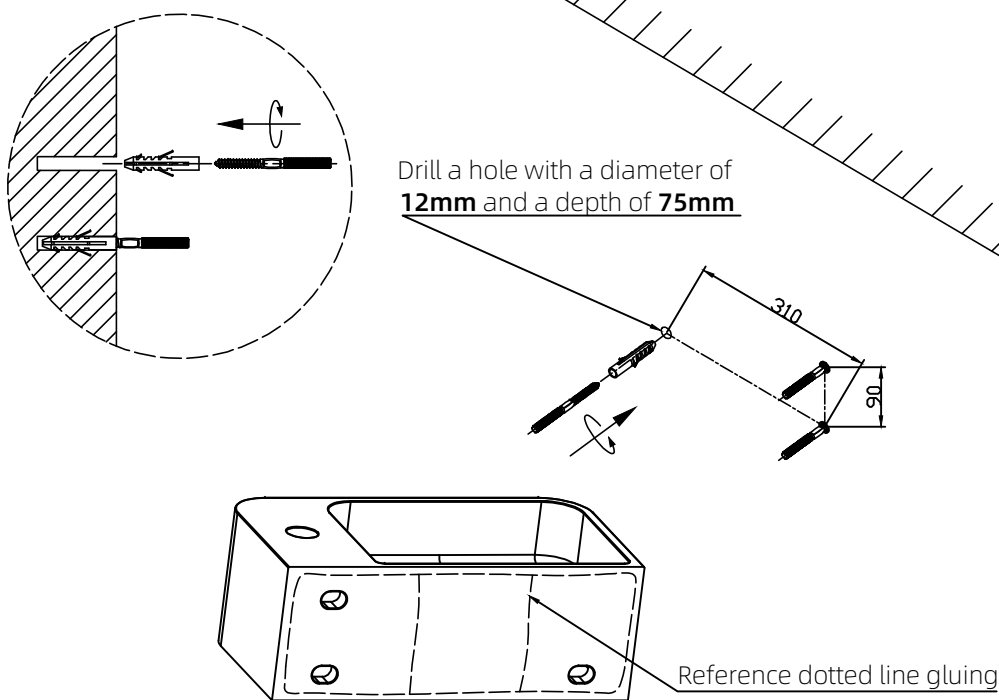
Concrete Basin x 1
